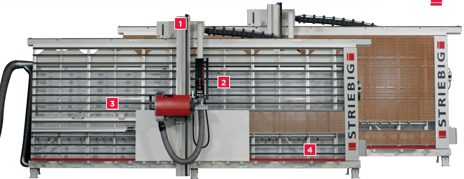
Illu: TWO VERSIONS – WIDE VARIETY OF POSSIBILITIES: TRK2 Automatically yielding aluminium support frame, TRK1 Automatically yielding wooden support wall.
